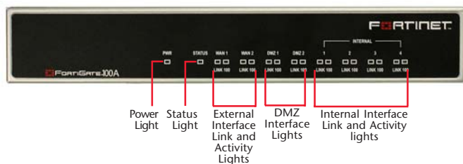
FortiGate-100A
